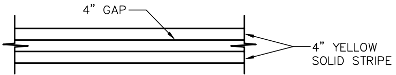
DOUBLE YELLOW CENTERLINE STRIPE
